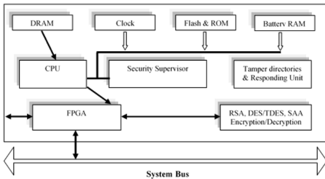
Fig. Crypto Coprocessor
